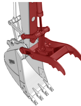
Hydraulic Strut Progressive Link
