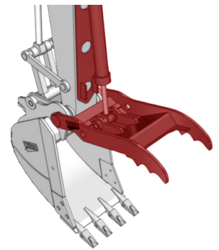
Hydraulic Strut Non-Link
