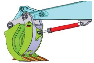
Hydraulic Strut 3 Over 2 Tine Jaw Configuration
