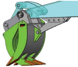
Manual Strut 2 Over 3 Tine Jaw Configuration
