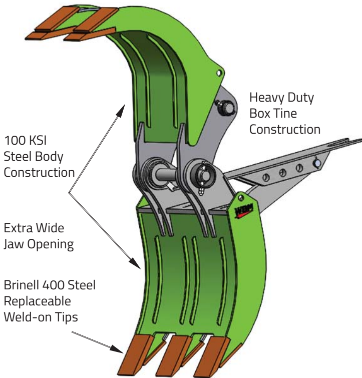
Manual Strut 2 Over 3 Tine Jaw Configuration
